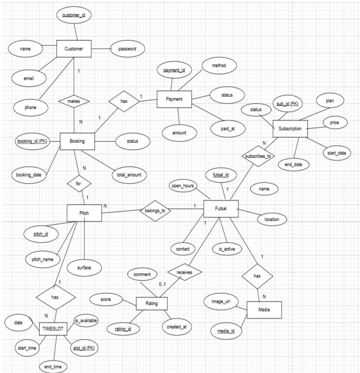
Figure 3.5 : Er Diagram 2
